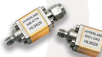
HL9429 / HL9529 110GHz Attenuator / Load
