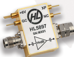
HL5897 63GHz Amplifier
