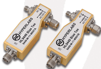
HL9449 110GHz Bias Tees
