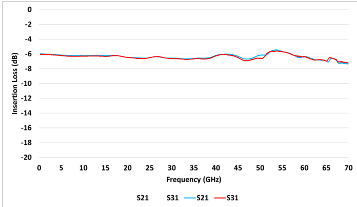
Figure 1: Typical HL9477 Bandwidth and Amplitude Match
