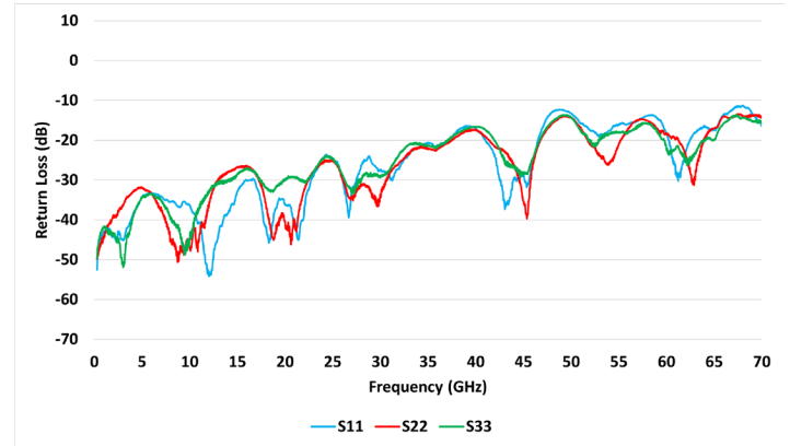
Figure 2: Typical HL9477 Return Loss
