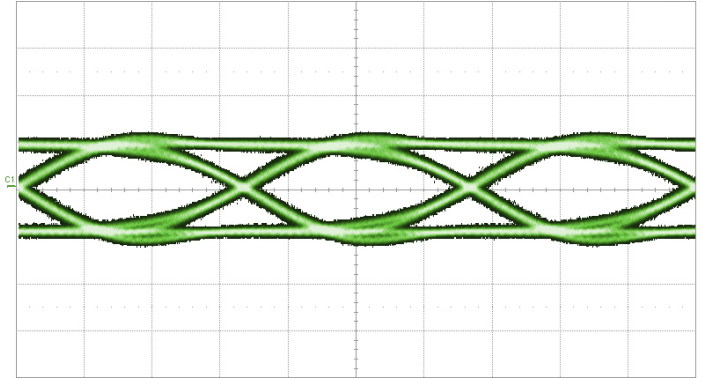
Figure 6: HL9477 56 Gbps PRBS 11, RF Output
