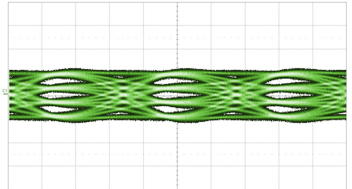
Figure 8: HL9477 112 Gbps PAM4, RF Output
