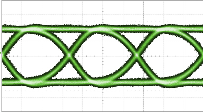
Figure 5: HL9477 56 Gbps PRBS 11, RF Input
