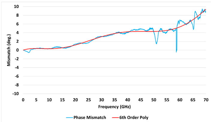
Figure 3: Typical HL9477 Phase Mismatch
