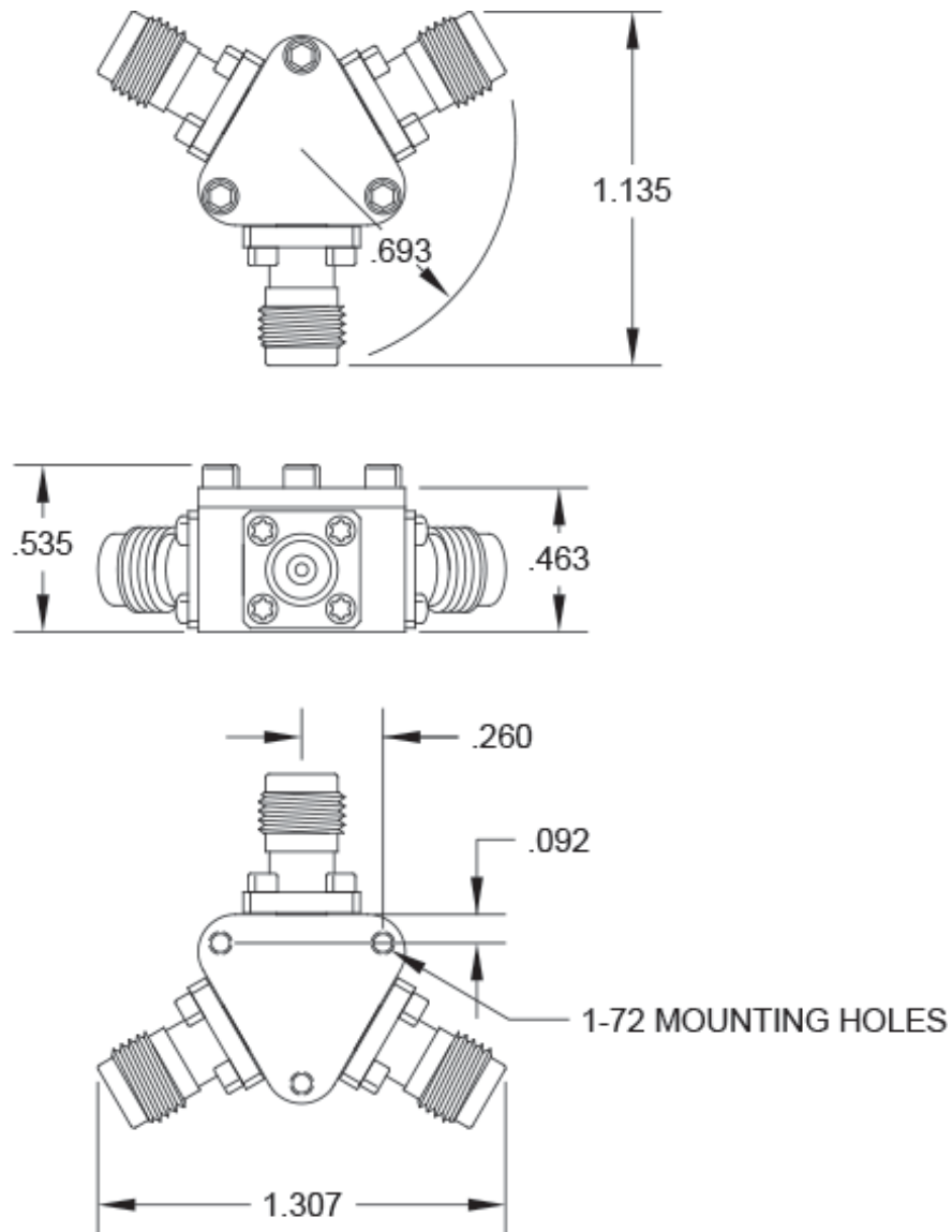
Figure 9: HL9477 Mechanical Drawing
