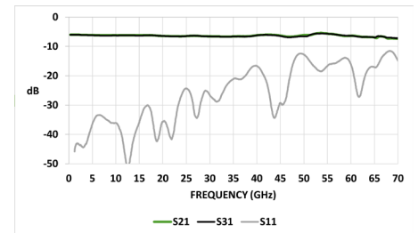
Typical HL9477 Insertion and Return Loss
