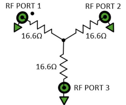
HL947x Schematic and Port Assignments
