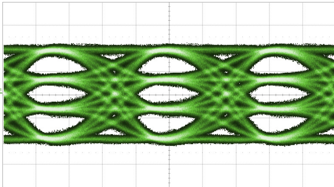
Figure 7: HL9477 112 Gbps PAM4, RF Input
