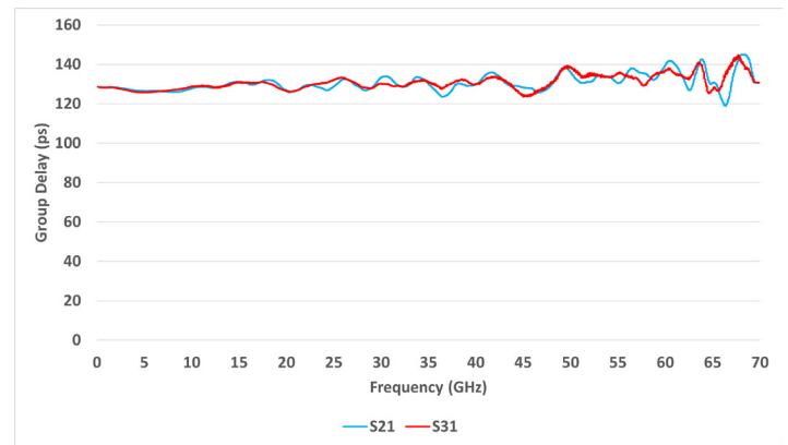
Figure 4: Typical HL9477 Group Delay
