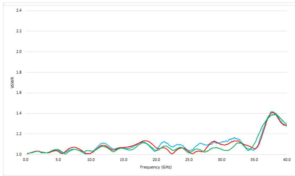
Figure 4: Typical VSWR on the HL9474
