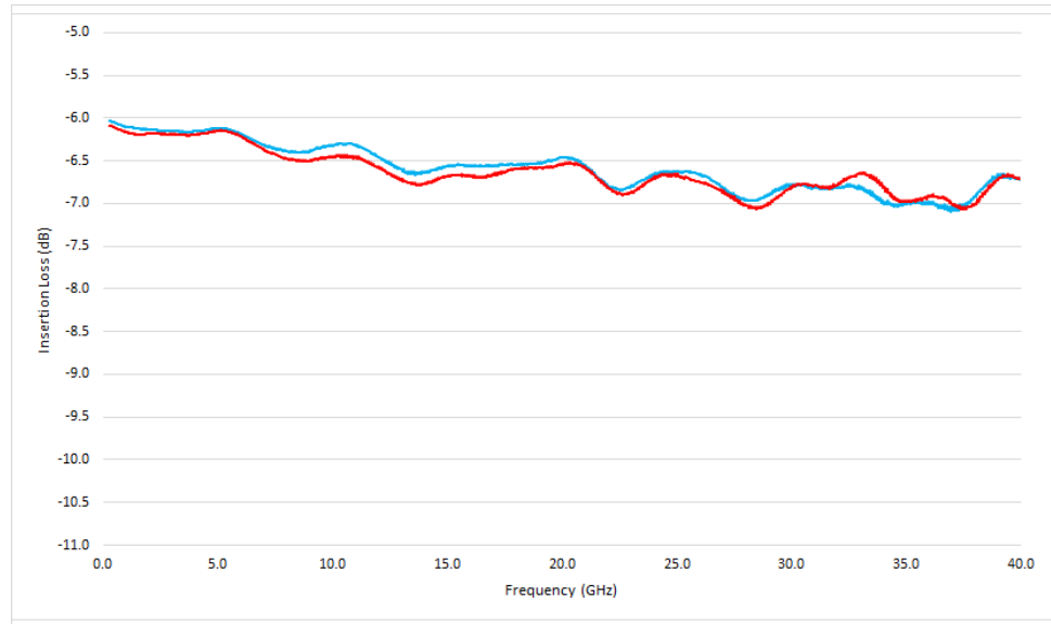
Figure 1: Typical amplitude match of an HL9474 device
