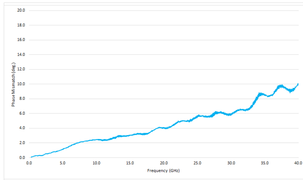
Figure 2: Typical phase mismatch of HL9474 output ports, in degrees
