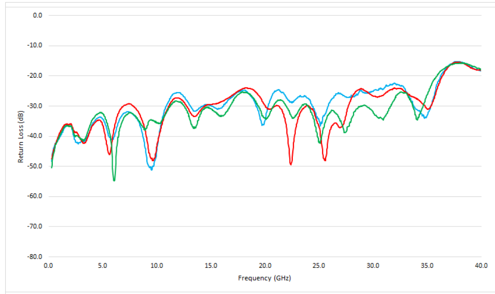
Figure 3: Typical return loss on the HL9474
