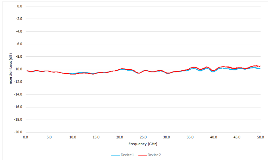
Figure 3: Typical HL9465 (opt. -M-JPJ) amplitude match along the thru line
