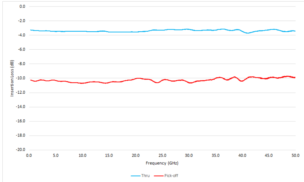
Figure 1: Typical insertion loss of the HL9465 (opt. -U-JPJ) along the thru and pick-off lines
