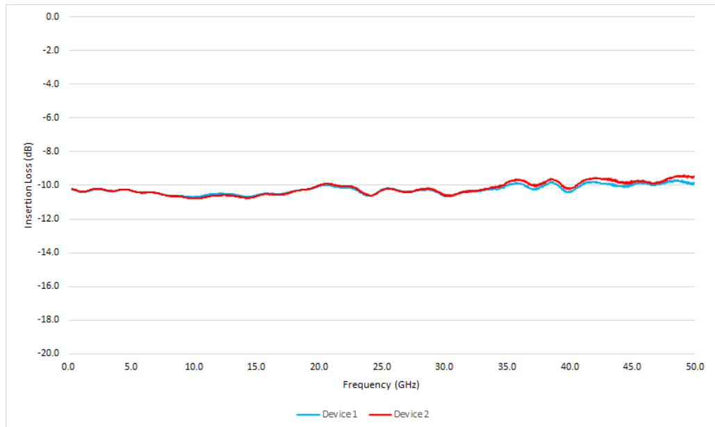
Figure 4: Typical HL9465 (opt. -M-JPJ) amplitude match along the pick-off line
