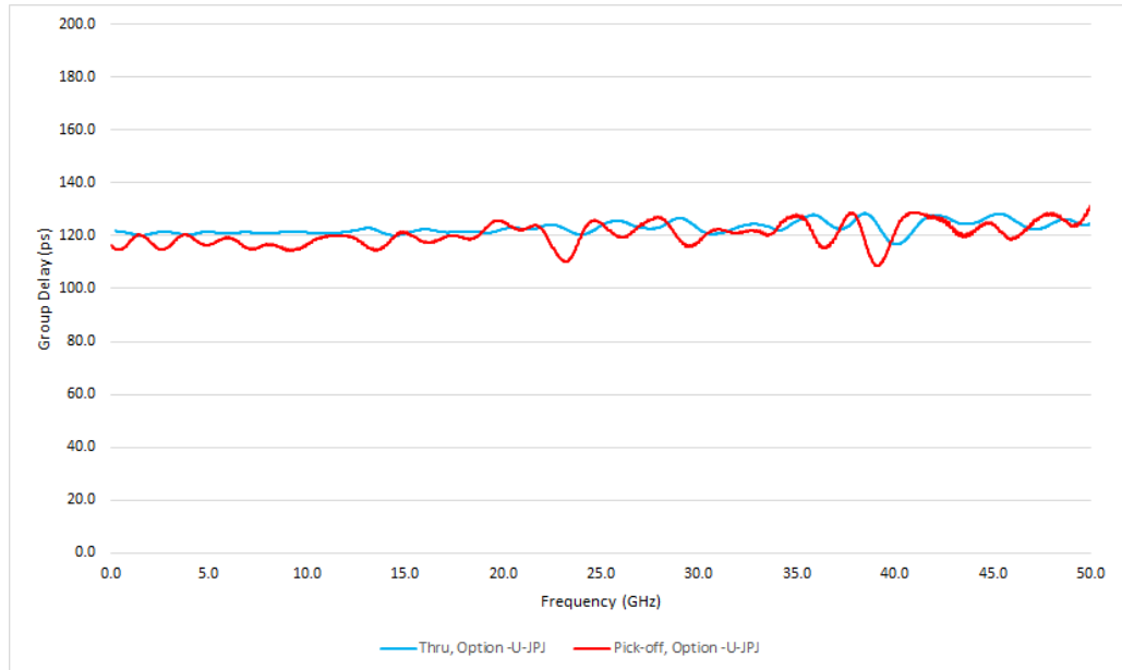
Figure 2: Typical group delay of the HL9465 (opt. -U-JPJ) along the thru and pick-off lines
