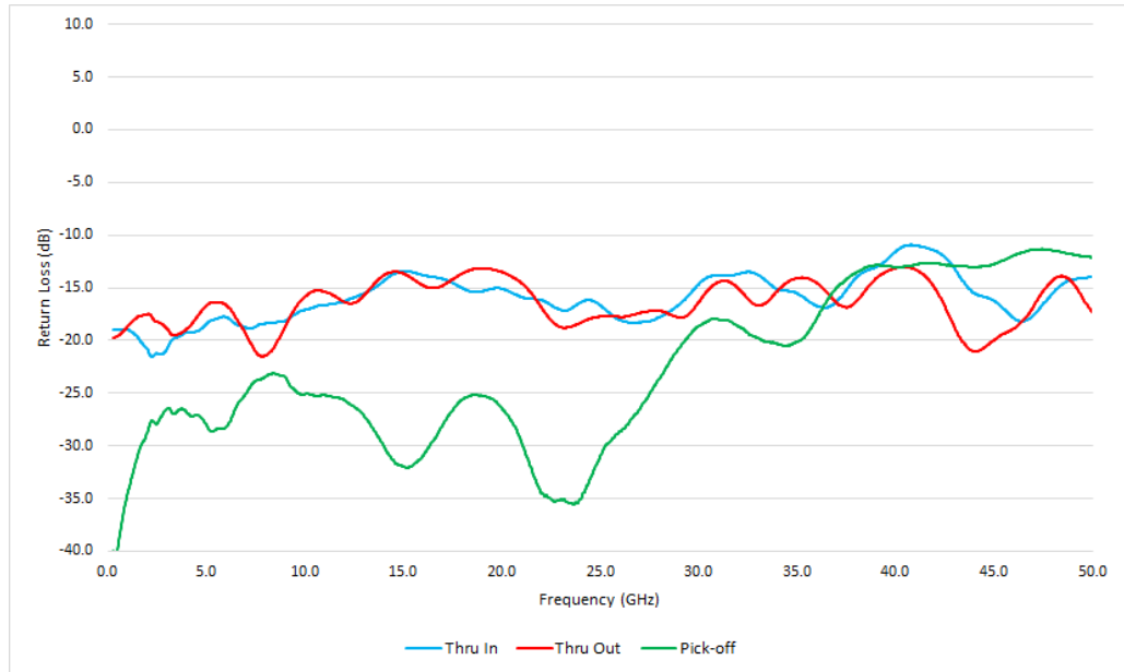
Figure 5: Typical HL9465 (opt. -U-JPJ) return loss on all ports
