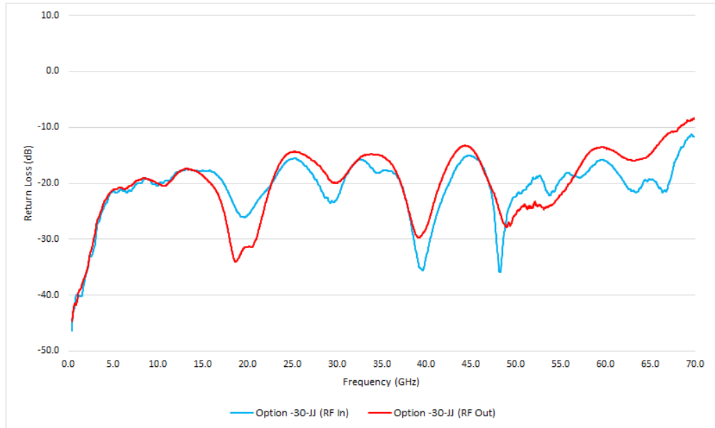
Figure 3: Typical HL9437 return loss, option -30-JJ
