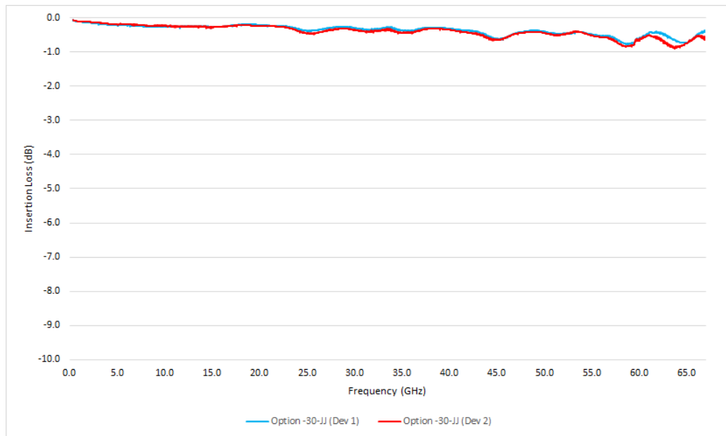
Figure 5: Typical HL9437 amplitude matched pair, option -30-JJ
