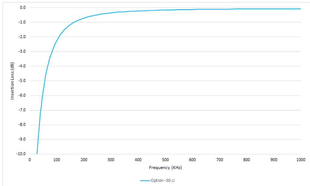
Figure 2: Typical HL9437 low-frequency performance, option -30-JJ
