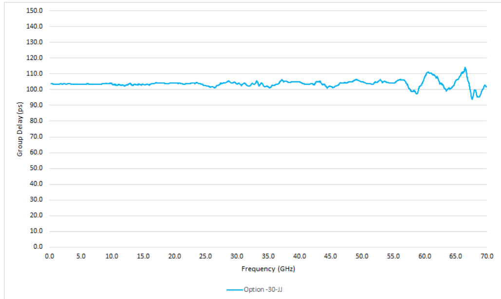
Figure 4: Typical HL9437 group delay, option -U-30-JJ
