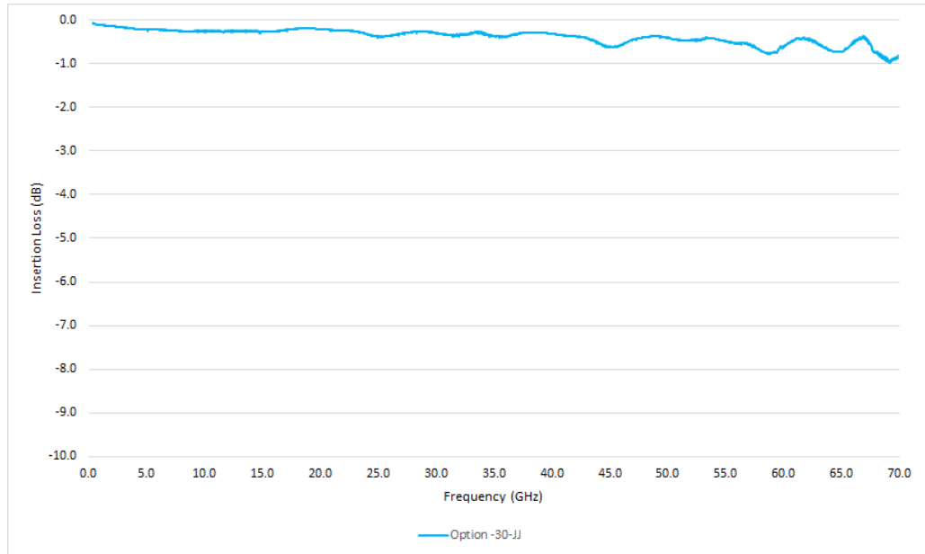
Figure 1: Typical HL9437 bandwidth and insertion loss, option -30-JJ
