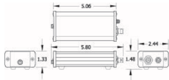
Figure 2: HL9101 dimensional drawing
